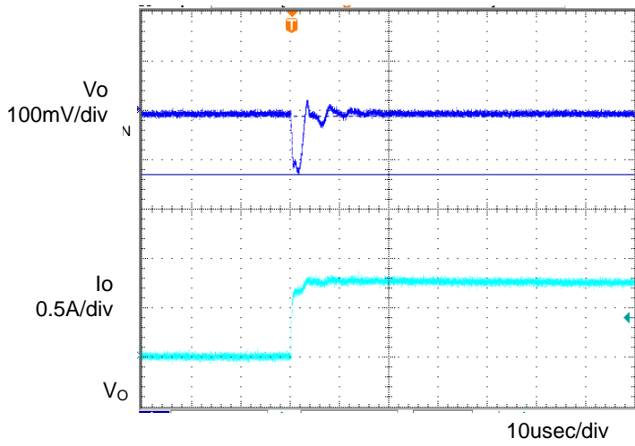
Figure 3. Transient Response (0→1.0A) Co=1µF, Ta=-40°C
