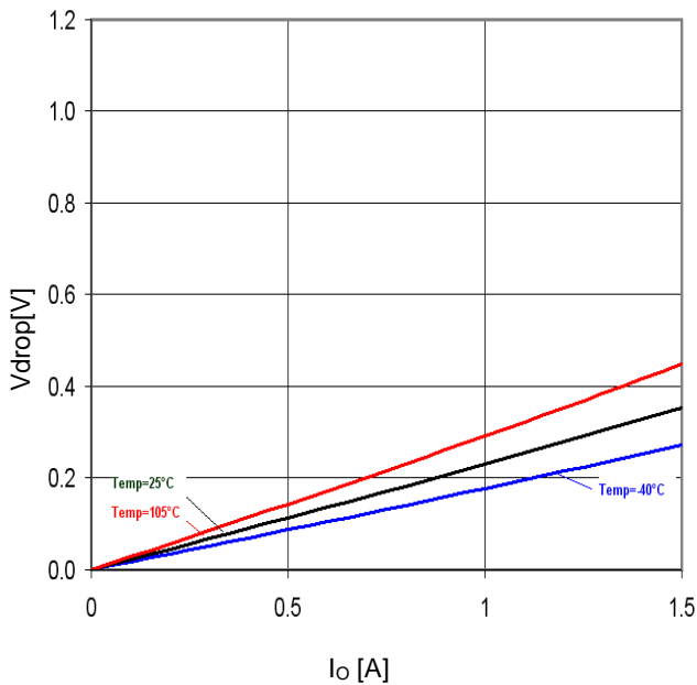
Figure 37. Minimum dropout Voltage 2 ( V_{CC}=10V , T_a=25^\circ C )
