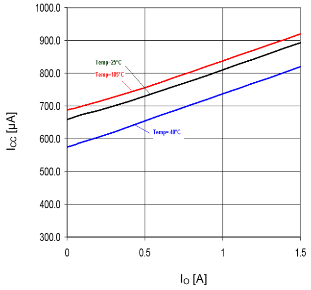
Figure 32. Io-Icc
