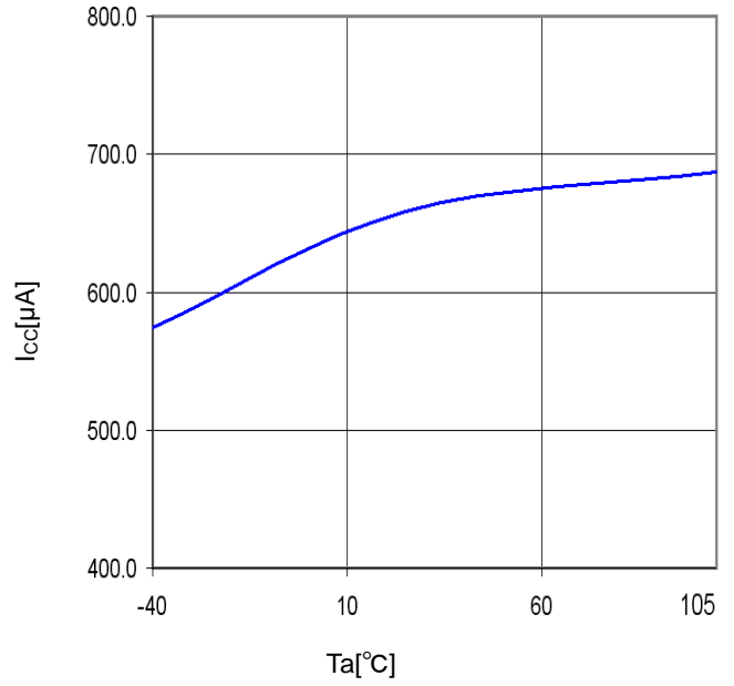
Figure 22. T_a - I_{cc}
