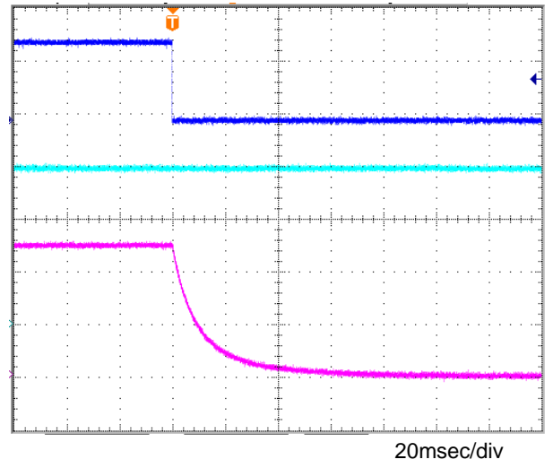
Figure 20. OFF sequence 2 C_o = 1\mu\text{F} , T_a = 105^\circ\text{C}
