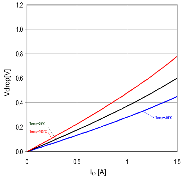
Figure 34. Minimum dropout Voltage 2 (VCC=4.5V、Ta=25°C)
