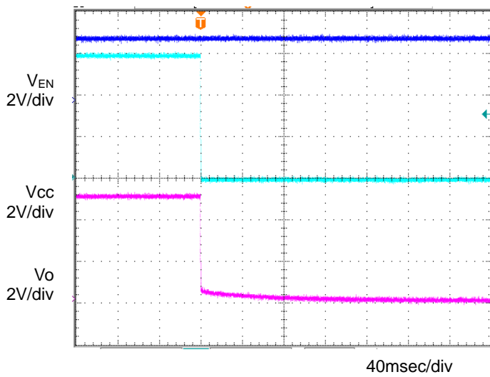
Figure 13. OFF sequence 1 Co=1μF, Ta=25°C
