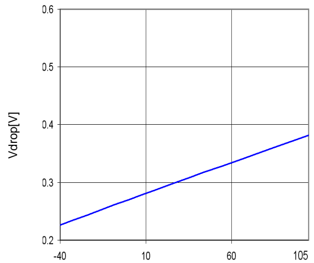
Figure 30. Minimum dropout Voltage1 ( V_{CC}=6\text{V} , I_o=1.0\text{A} )
