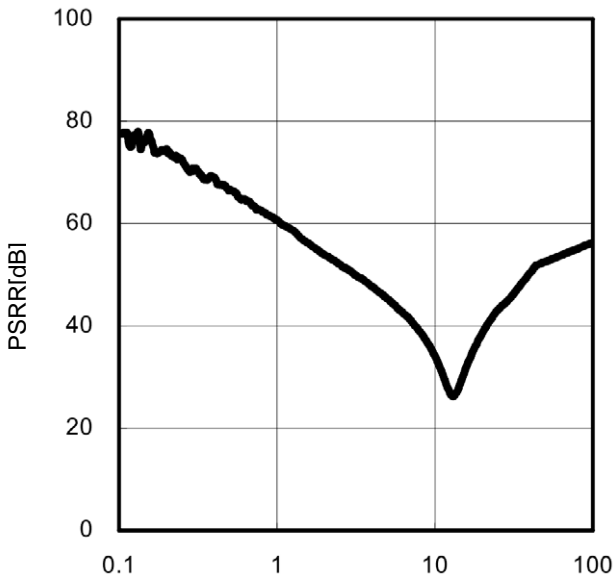
Figure 33. PSRR(Io=0mA)
