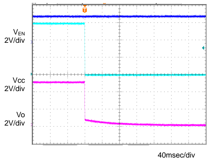
Figure 12. OFF sequence 1 Co=1μF, Ta=-40°C
