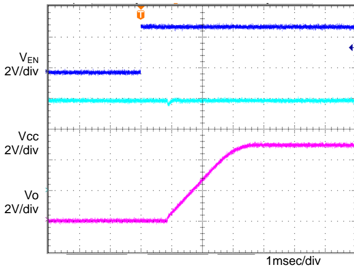
Figure 17. Input sequence 2 Co=1μF, Ta=105°C
