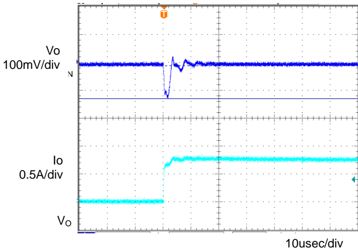
Figure 3. Transient Response (0→1.0A) Co=1μF, Ta=-40°C
