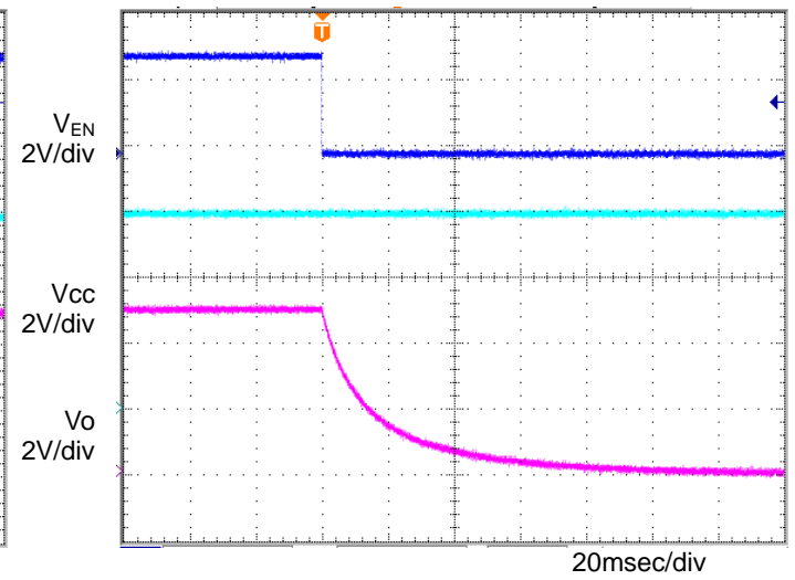
Figure 18. OFF sequence 2 Co=1μF, Ta=-40°C
