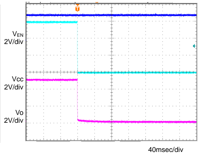
Figure 14. OFF sequence 1 Co=1μF, Ta=105°C
