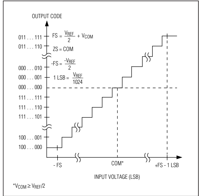
Figure 9. Bipolar Transfer Function, Full Scale (±FS) = ±VREF/2
