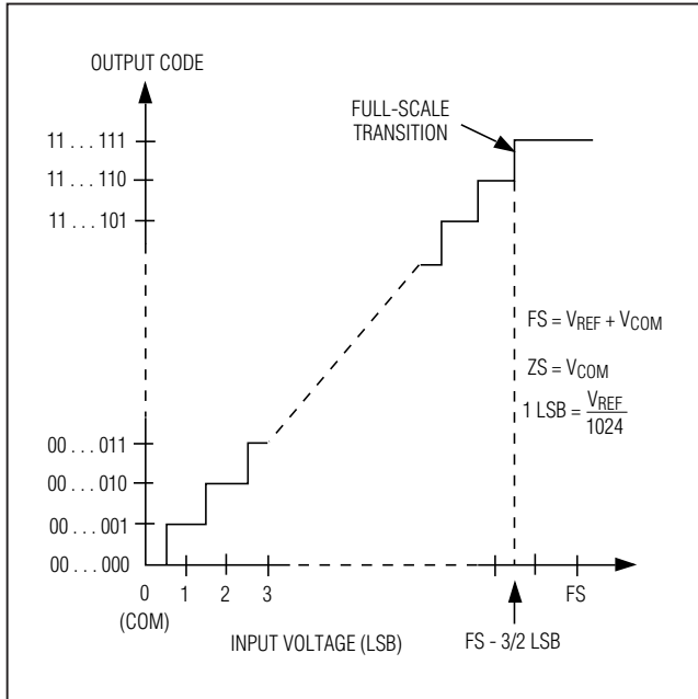
Figure 8. Unipolar Transfer Function, Full Scale (FS) = V REF
