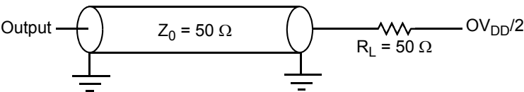
Figure 7. Local Bus AC Test Load
