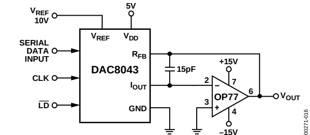
Figure 16. Unipolar Operation with High Accuracy Op Amp (2-Quadrant)
