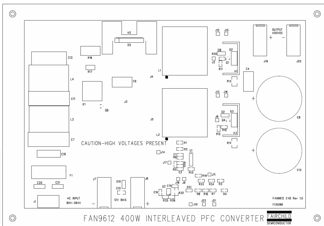
Figure 13. Top Silkscreen
