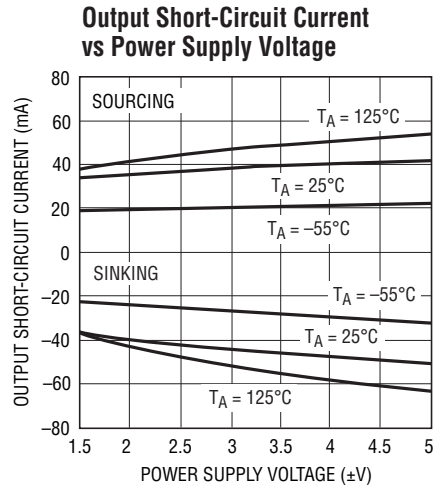
LT6202/03/04 G11
