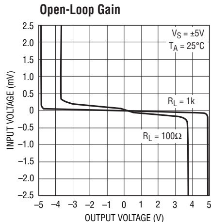
LT6202/03/04 G14
