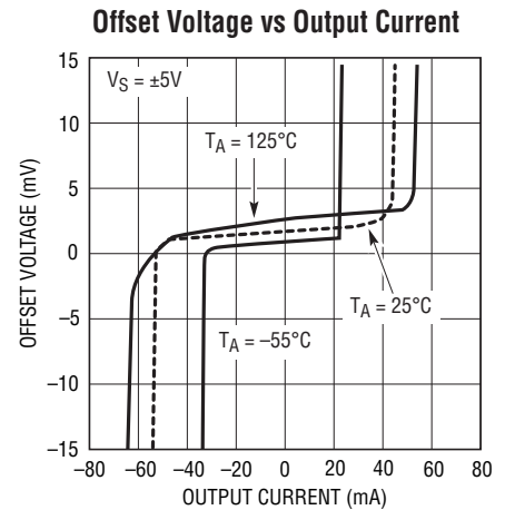
LT6202/03/04 G15
