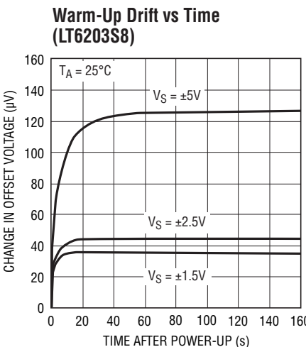
LT6202/03/04 G16
