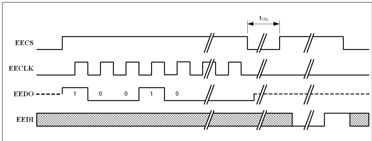
FIGURE 10-3: EEPROM ERASE ALL CYCLE
