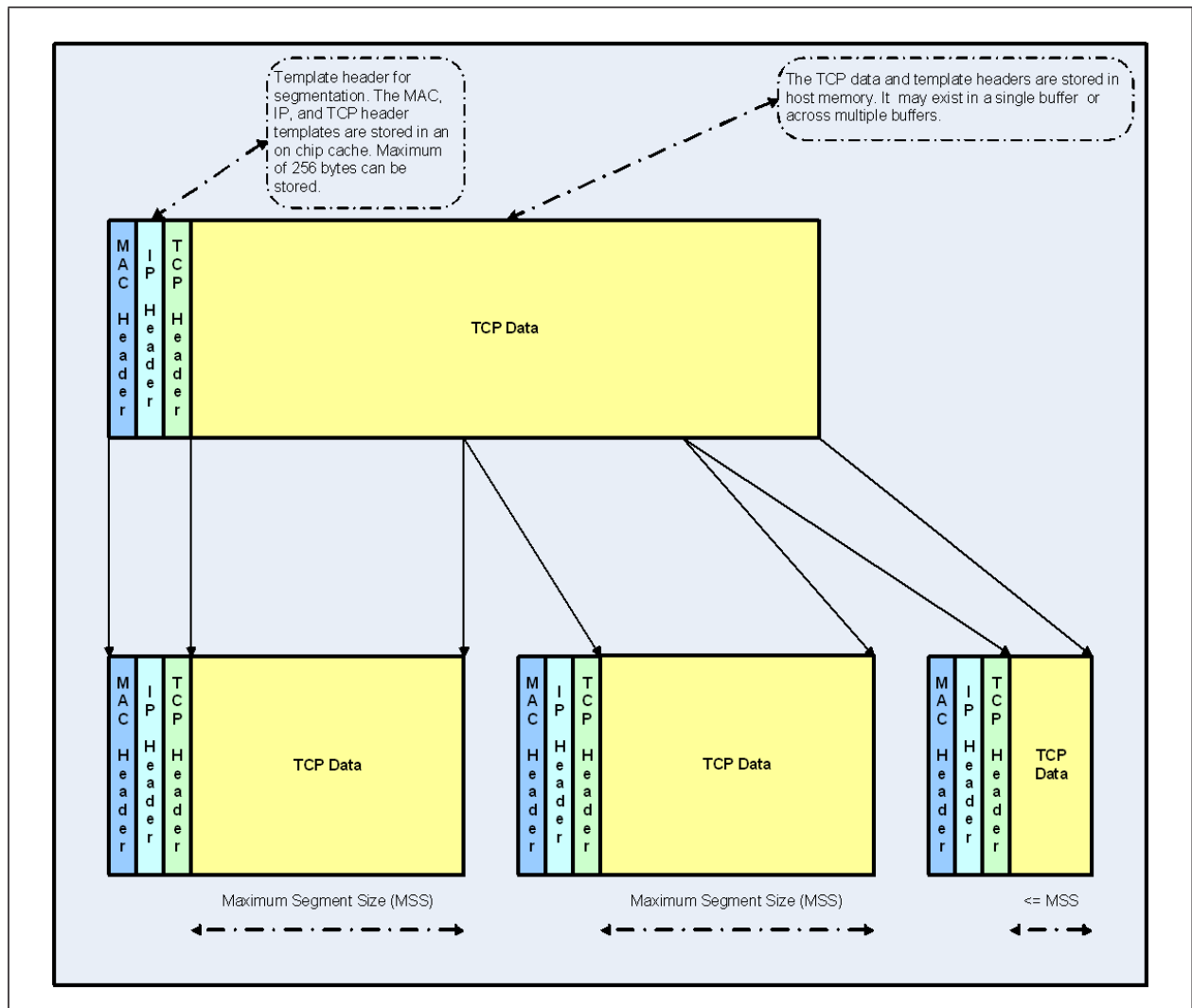
FIGURE 6-4: TCP SEGMENTATION
