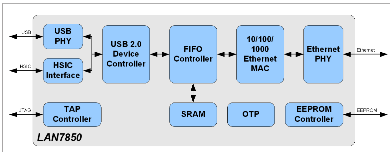
FIGURE 2-1: INTERNAL BLOCK DIAGRAM
