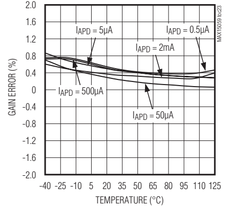
GAIN ERROR vs. TEMPERATURE (MAX15059A)
