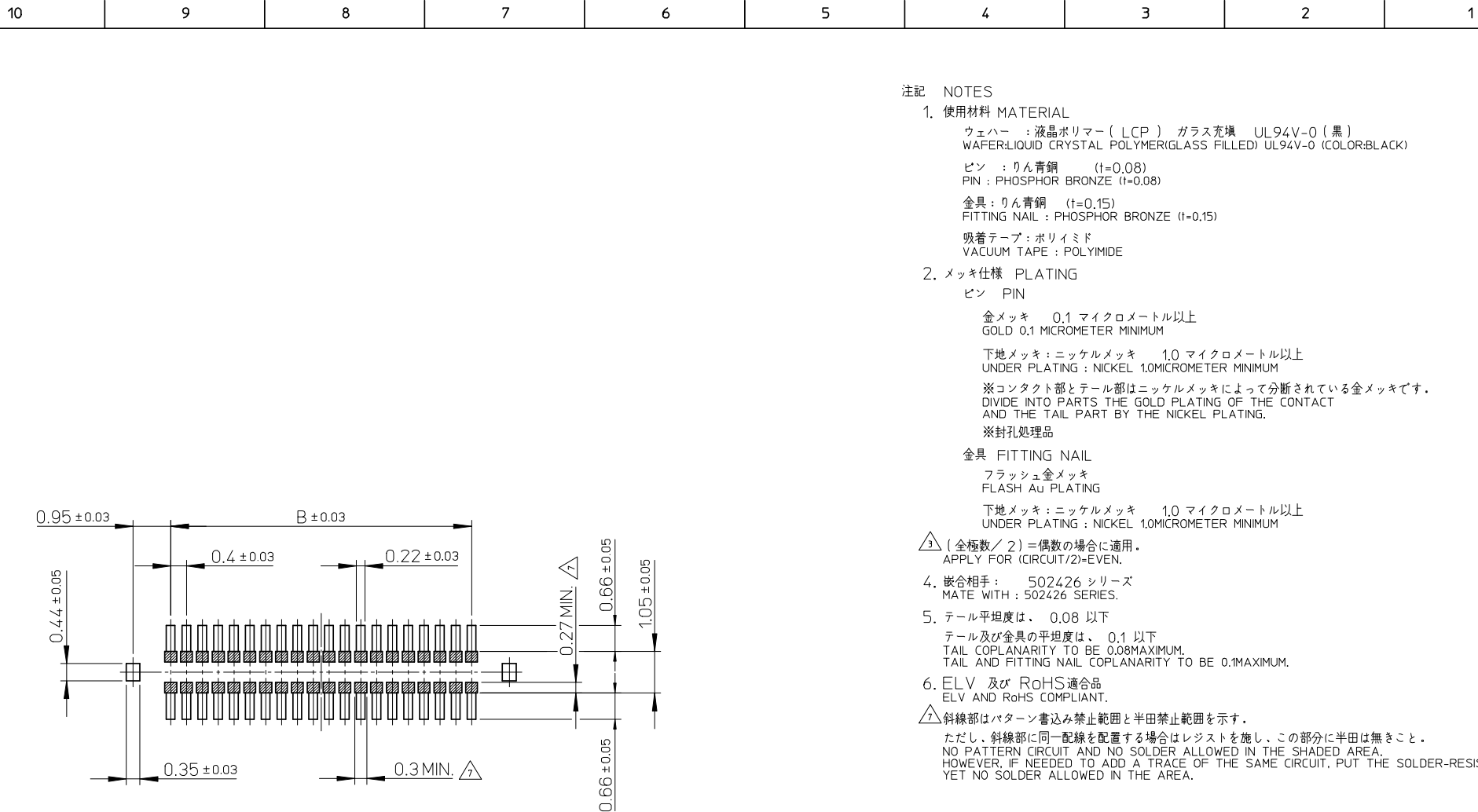
P.C. BOARD PATTERN LAYOUT (REFERENCE)
