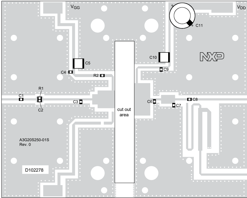
Figure 2. A3G20S250-01SR3 Test Circuit Component Layout
