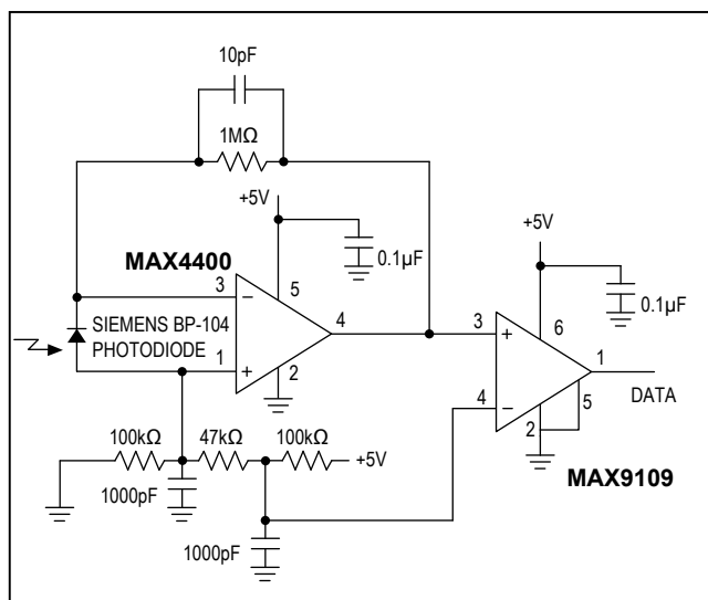
Figure 4. Battery-Operated Infrared Data Link Consumes Only 760µA
