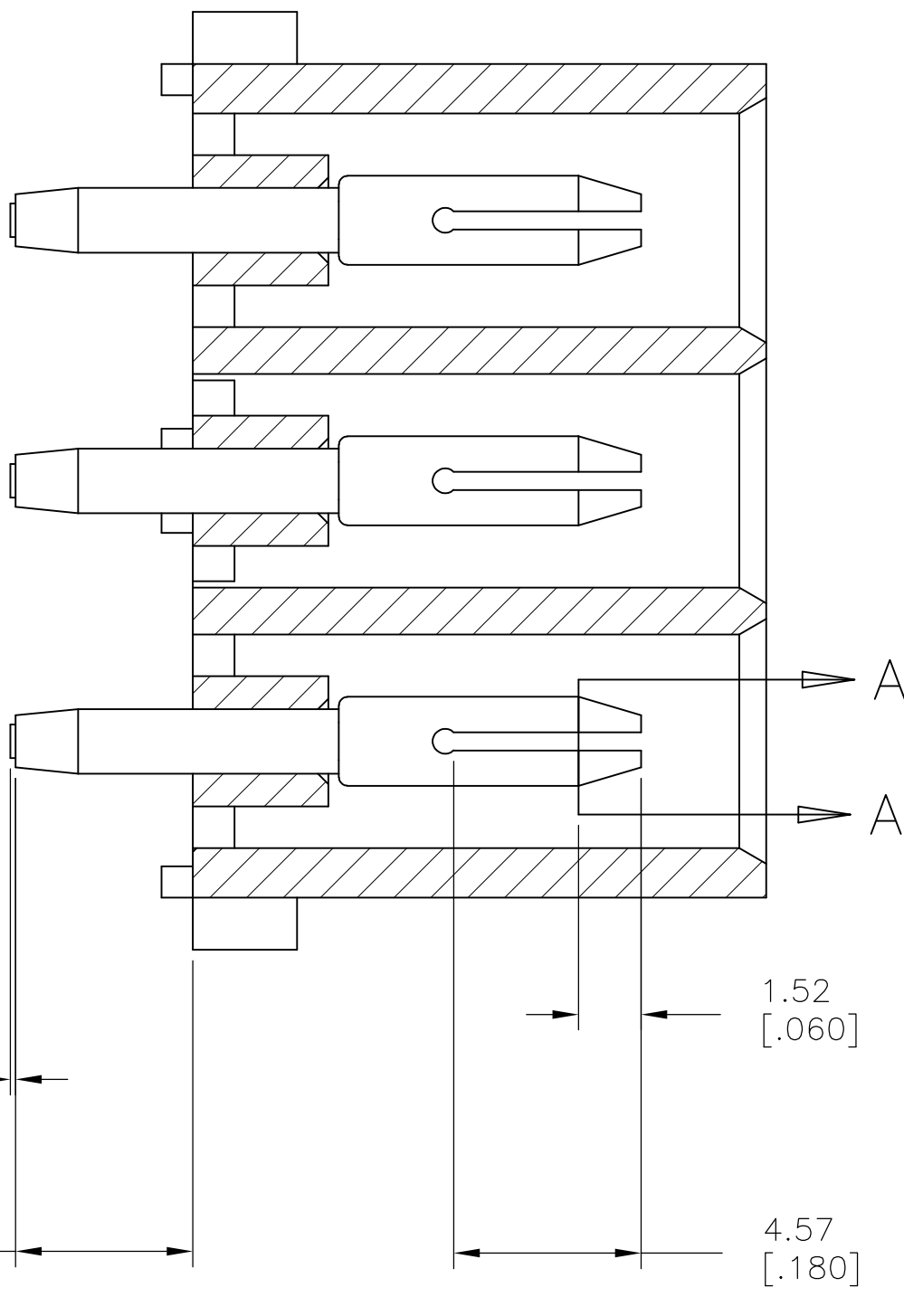
SECTION B-B
