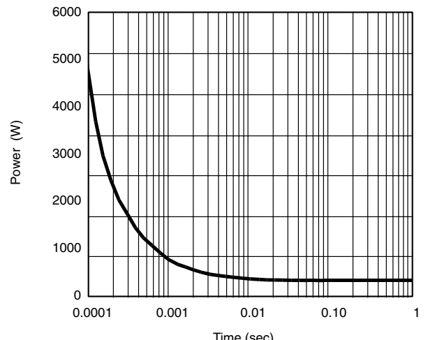
Single Pulse Power, Junction-to-Case ( T_C = 25\text{ °C} )
