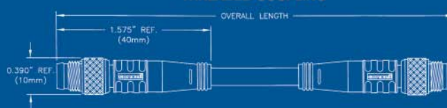
STRAIGHT/90° MALE/FEMALE DOUBLE ENDED THREADED COUPLING
