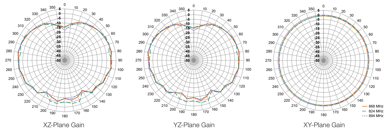
Figure 8. Radiation Patterns for CW LTE Band 5 Antenna
