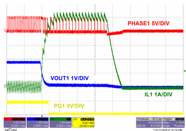
FIGURE 27. OUTPUT SHORT CIRCUIT CHANNEL 1
