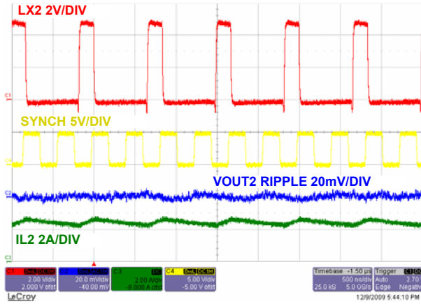
FIGURE 24. STEADY STATE OPERATION CHANNEL 2 AT FULL LOAD WITH F_{SW} = 2.4MHz
