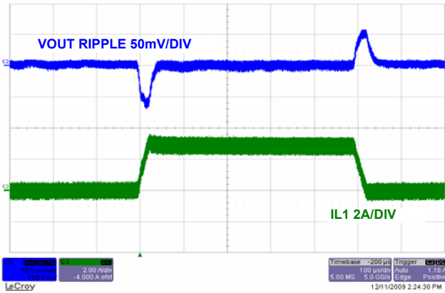
FIGURE 54. LOAD TRANSIENT CHANNEL 1
