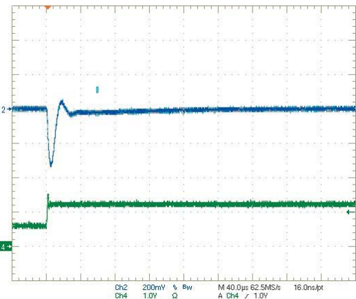
Step Load Transient Response ( V_{IN} = 5V , V_{OUT} = 2.5V , I_{OUT} = 3A to 6A) Trace 2=Vout, 200 mV/div. Trace 4=Iout, 5A/div.
