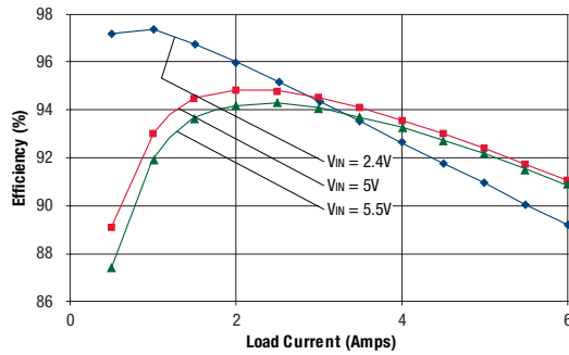
Efficiency vs. Line Voltage and Load Current @ +25°C ( V_{OUT} = 1.8V )
