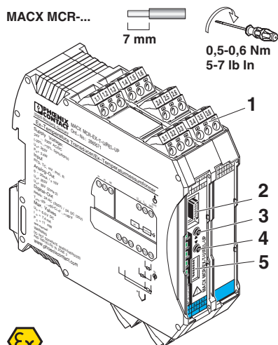
Figure 4 Structure MACX MCR-EX-T-UIREL-UP
