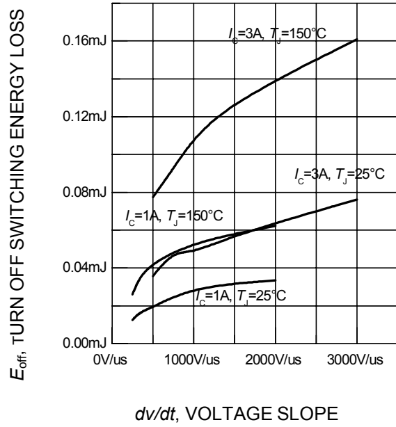
Figure 16. Typical turn off switching energy loss for soft switching
