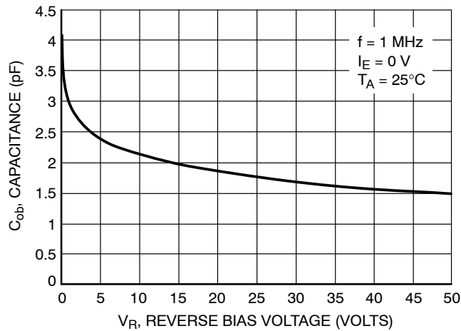
Figure 49. Output Capacitance
