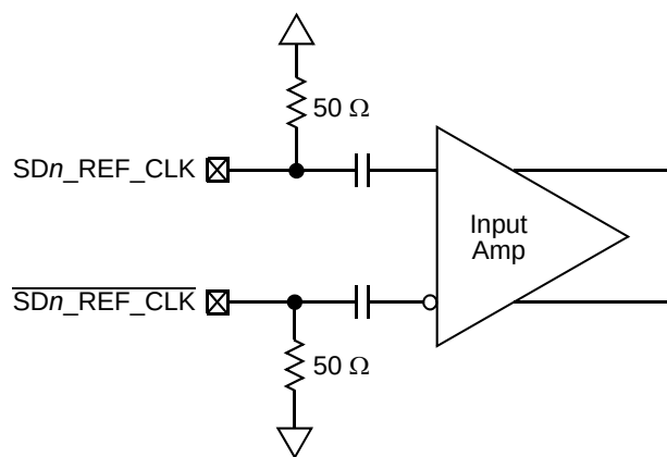
Figure 23. Receiver of SerDes Reference Clocks
