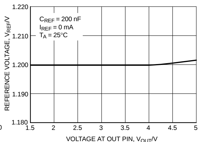
Figure 3. Reference Voltage vs. Voltage at OUT Pin
