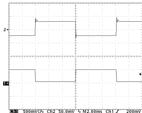
( V_{OUT} = 3.3\text{ V} , I_{LOAD} = 50\text{ mA to }500\text{ mA} ; L = 5.6\text{ }\mu\text{H} , C_{OUT} = 22\text{ }\mu\text{F} ) Upper Trace: Output Voltage Ripple, 50 mV/Division Lower Trace: Load Current, I_{LOAD} , 500 mA/Division
