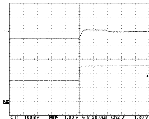
( V_{IN} = 1.5\text{ V to }2.5\text{ V} ; L = 5.6\text{ }\mu\text{H} , C_{OUT} = 22\text{ }\mu\text{F} , I_{LOAD} = 100\text{ mA} ) Upper Trace: Output Voltage Ripple, 100 mV/Division Lower Trace: Battery Voltage, V_{IN} , 1.0 V/Division
