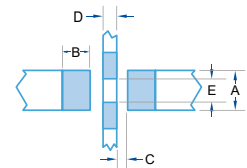
Recommended solder lands
