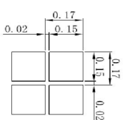
CONSECC Layout
