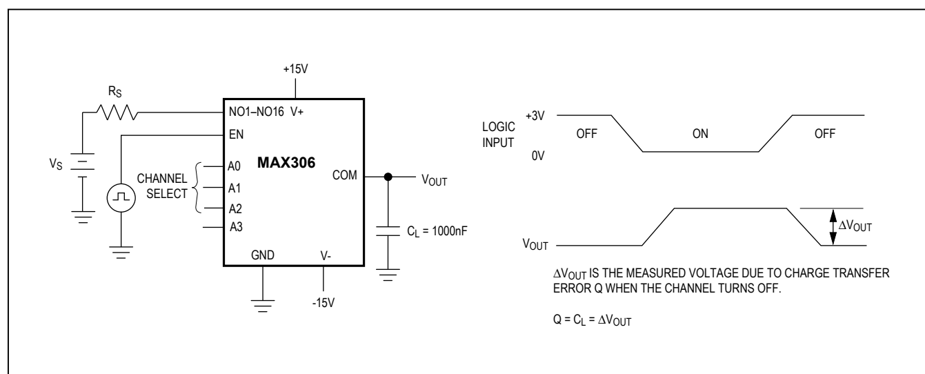
Figure 5. Charge Injection
