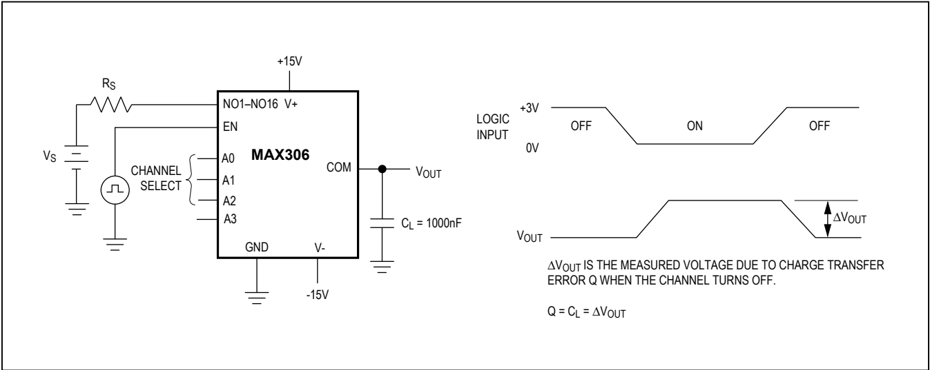
Figure 5. Charge Injection
