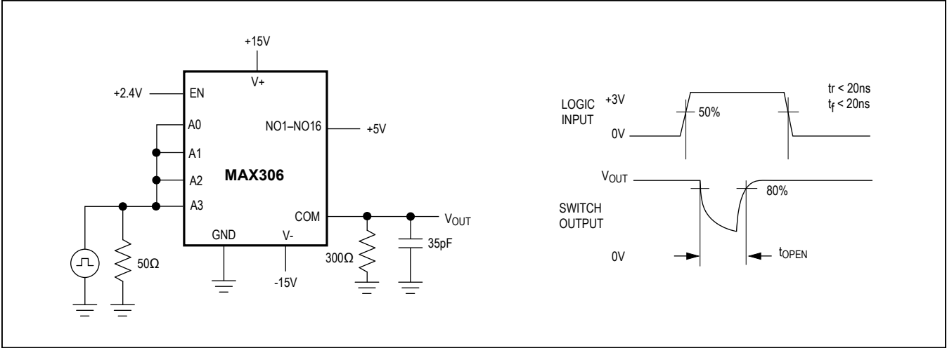
Figure 4. Break-Before-Make Interval
