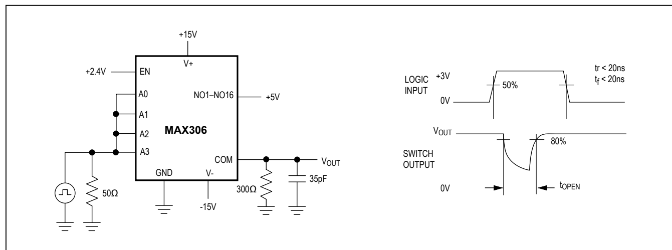
Figure 4. Break-Before-Make Interval
