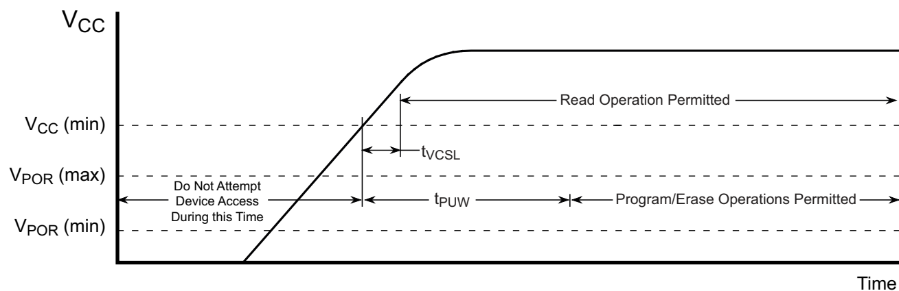
Figure 16-1. Power-Up Timing
