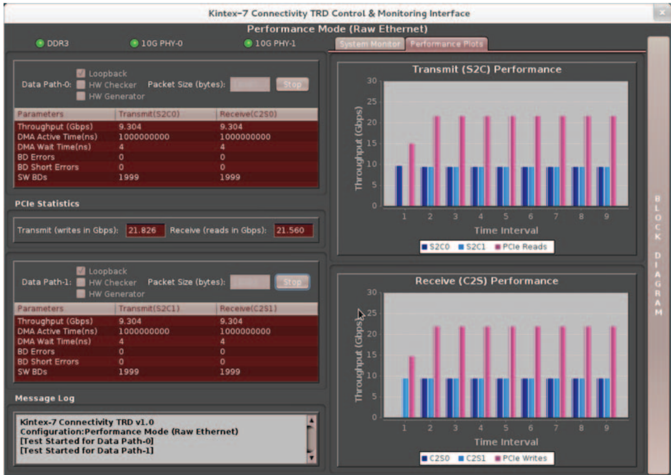
Figure 2-24: Raw Ethernet Driver Performance Plots
