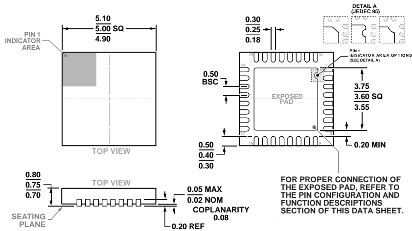
COMPLIANT TO JEDEC STANDARDS MO-220-WHHD-5 Figure 25. 32-Lead Lead Frame Chip Scale Package [LFCS] 5 mm × 5 mm Body and 0.75 mm Package Height (CP-32-12) Dimensions shown in millimeters
