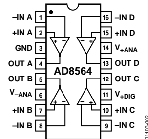
Figure 3. 16-Lead PDIP (N-16)
