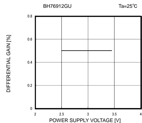
Fig. 45 Differential Gain vs Supply Voltage
