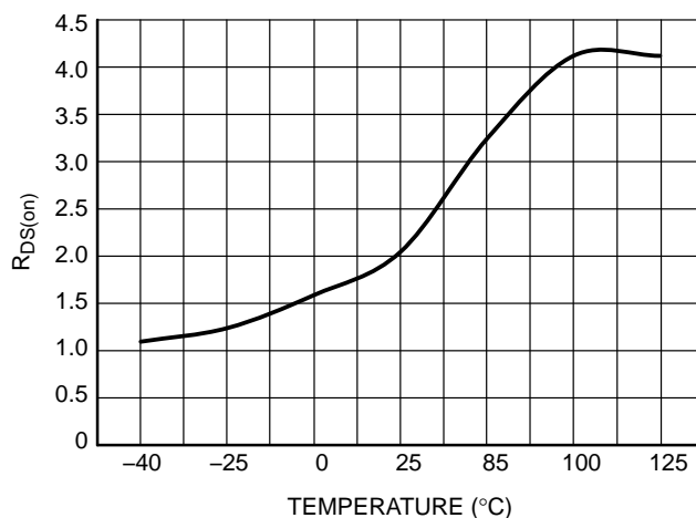
Figure 32. NCP 1129 R DS(on) vs. Junction Temperature
