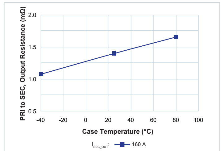
Figure 9 — R_{OUT} vs. temperature; Nominal V_{PRI\_DC} I_{SEC\_DC} = 160\text{ A} at T_{CASE} = 80^{\circ}\text{C}
