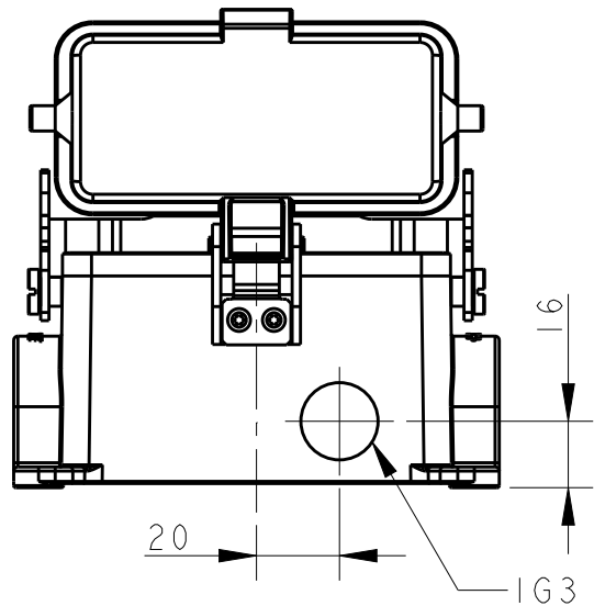
TYPE 3: BODY + STEEL LOCKING + PLASTIC PROTECTION COVER 1 SIDE ENTRY + 1 FRONT ENTRY OTHER SPEC REFER TO TYPE 2
