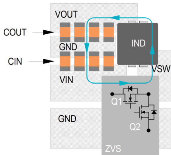
Figure 23 - Recommended component placement and metal routing
