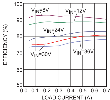
Load Efficiency
