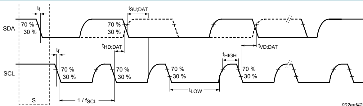
Figure 16. I 2 C-bus pins clock timing
