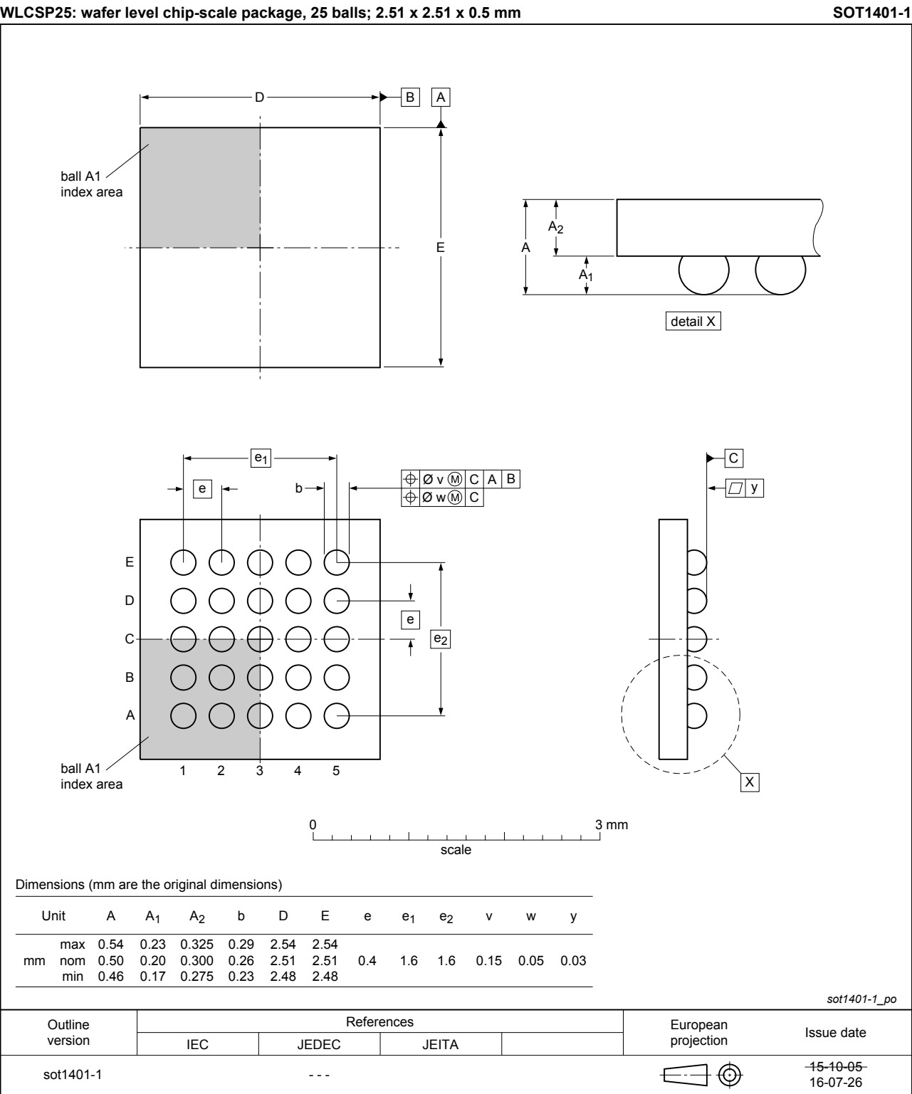
Figure 20. WLCSP25 package outline
