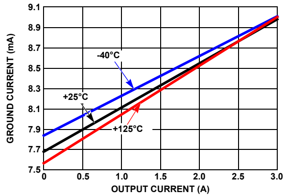
FIGURE 8. GROUND CURRENT vs OUTPUT CURRENT
