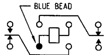
TERMINAL VIEW
