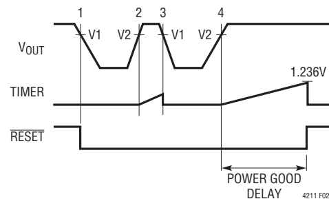
Figure 2. Supply Monitor Waveforms in Normal Mode
