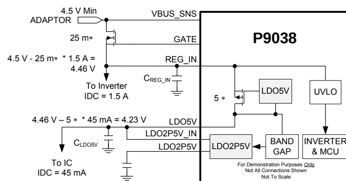
Figure 2. Input Voltage Support Range (UVLO)
