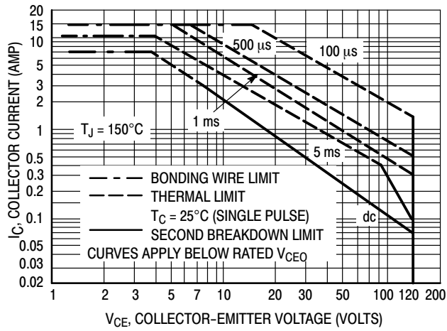
Figure 12. Maximum Forward Bias Safe Operating REA
