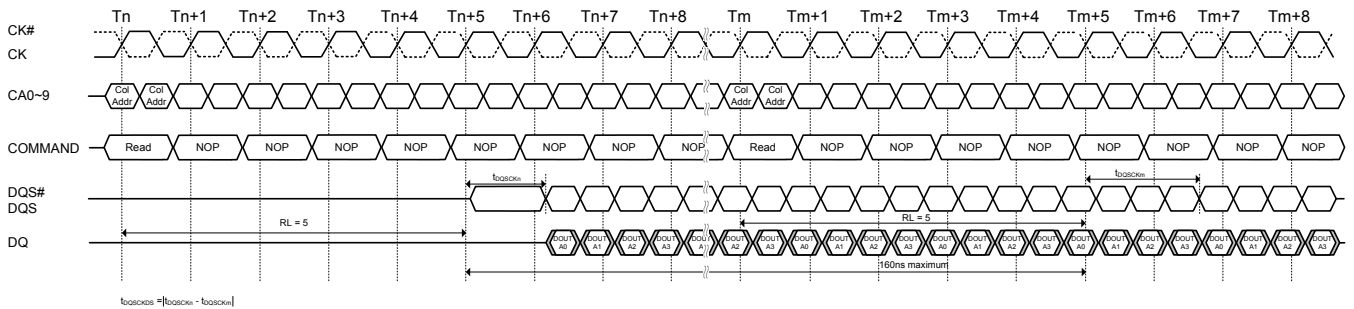
Figure 17. tDQCKDS timing
