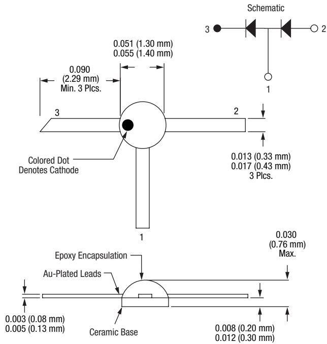
Figure 12. -232 Package Dimensions
