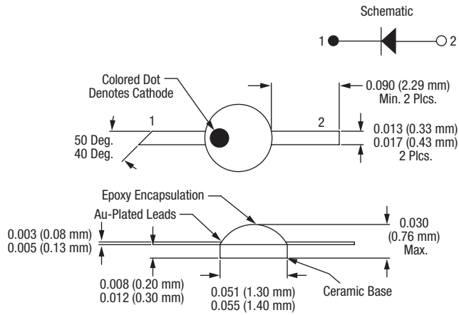
Figure 11. -230 Package Dimensions
