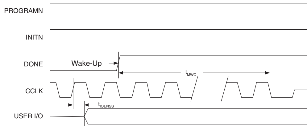
Figure 3-27. Wake-Up Timing
